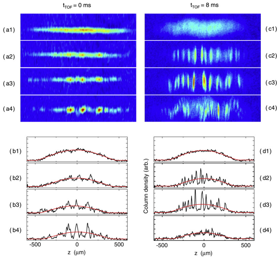
Fig. 4. In situ profiles and TOF matter wave interference of disordered BEC. (a1–a4) In situ images for V_D/\mu \approx 0, 0.3, 0.5 and 1.0 , respectively; (b1–b4) In situ column-density profiles (axial cuts for images a1–a4); (c1–c4) TOF images taken 8 ms after releasing the BEC, for V_D/\mu \approx 0, 0.3, 0.5 and 1.0 , respectively; (d1–d4) TOF column-density profiles (axial cuts for images c1–c4). Solid red lines are fits to Thomas–Fermi distributions. \omega_2 \approx 2\pi \times 2.8 Hz for data shown here. The TOF 2D image uses a different color scale from the one used for the in situ 2D image, and the displayed aspect ratio of the in situ 2D image is reduced by 50% in order to enhance the transverse size for visibility. Part of figure adapted from [21]. (For interpretation of the references to colour in this figure legend, the reader is referred to the web version of this article.)
