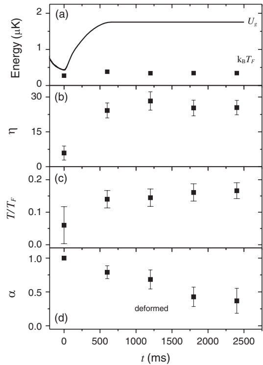
FIG. 5. Recompression of the trap following the 1 s evaporation. Here, the 1 s evaporation finishes at t = 0 and is followed by a slow recompression of the trap over the next 0.6 s. Even though the final value of U_g is similar to that shown for the 3.4 s trajectory in Fig. 3, the recompressed values of T_F are lower due to smaller overall numbers ( \sim 3 \times 10^4 vs \sim 10^5 ).
