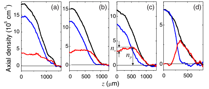
FIG. 2 (color online). Axial densities taken at various times t along the evaporation trajectory. The global polarizations P are (a) 600 ms, P = 0.14 , (b) 700 ms, P = 0.21 , (c) 740 ms, P = 0.28 , (d) 1 s, P = 0.18 . The variation in P is a result of shot-to-shot variations, as each image requires the trap to be reloaded and evaporated to the specified t . The upper (black) curves correspond to the majority state ( |\uparrow\rangle ), the middle (blue) curves to the minority state ( |\downarrow\rangle ), and the axial spin densities ( |\uparrow\rangle - |\downarrow\rangle ) are given by the lower (red) curves.
