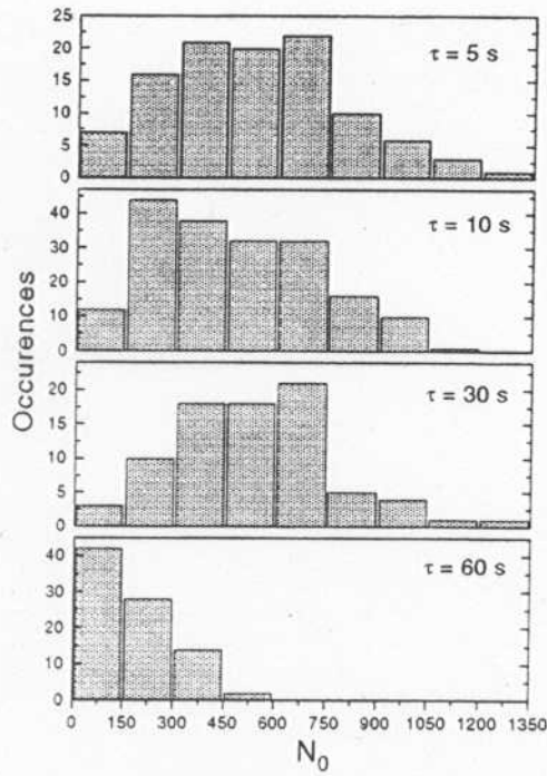
FIGURE 5. Frequency of occurrence of condensate occupation number. For each measurement, a nonequilibrium degenerate gas was produced, allowed to evolve freely for time \tau , and then probed. The spread in N_0 values arises as the collapse/fill cycle is sampled at random points.
