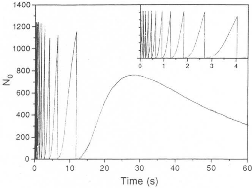
FIGURE 2. Numerical solution of the quantum Boltzmann equation, showing evolution of condensate occupation number. A trapped, degenerate {}^7\text{Li} gas is cooled at t = 0 to a temperature of about 100 nK and a total number of 4 \times 10^4 atoms. The gas then freely evolves in time. The inset shows an expanded view of the early time behavior on the same vertical scale.
