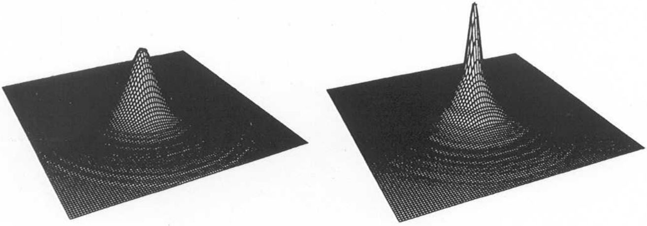
FIGURE 4. Phase-contrast images averaged around the cylindrical axis of the trap. For both cases, N \approx 23,000 atoms and T \approx 190 nK. For the image on the right, N_0 \approx 1050 , while for the image on the left N_0 \approx 65 . These images demonstrates our sensitivity to a small number of condensate atoms on a background of a large number of non-condensed atoms.
