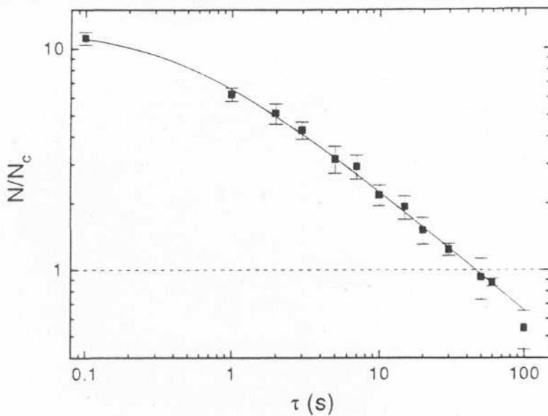
FIGURE 6. Relaxation of degenerate gas to equilibrium. Data were taken as in Fig. 5, but for each image the total number of atoms N and the temperature T were used to determine N/N_c , where N_c = 1.2(kT/\hbar\omega)^3 . Points represent averages of several measurements, and error bars are standard deviations. The dashed line at N/N_c = 1 approximately denotes the point at which equilibrium is reached. The solid curve is a fit to the empirical form A(1 + \kappa\tau)^\gamma , yielding A = 12 \pm 1 , \kappa = 2.1 \pm .7 \text{ s}^{-1} , and \gamma = -.55 \pm .03 .
