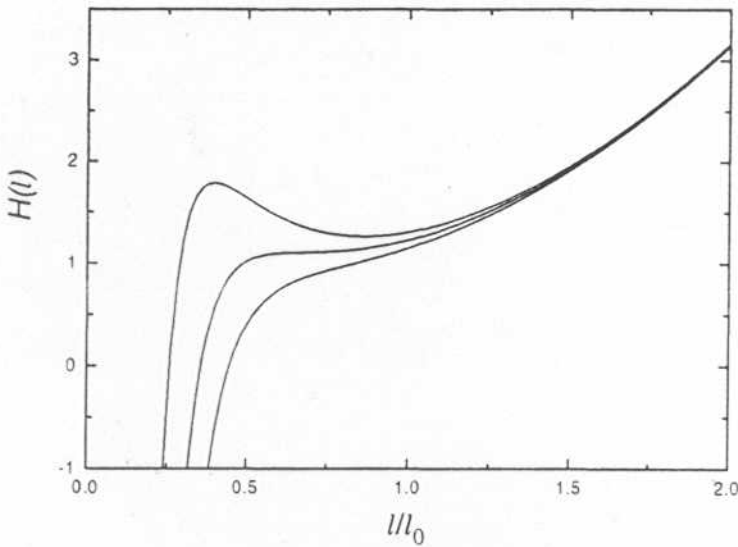
FIGURE 1. The condensate energy H , plotted in units of N_0 \hbar^2 / ml_0^2 . The upper curve corresponds to N_0 = 0.48 l_0 / |a| , the middle curve to N_0 = 0.68 l_0 / |a| , and the lower curve to N_0 = 0.87 l_0 / |a| . It is evident that a local minimum in H exists near l = l_0 if N_0 is sufficiently low, indicating that a metastable condensate can exist.
